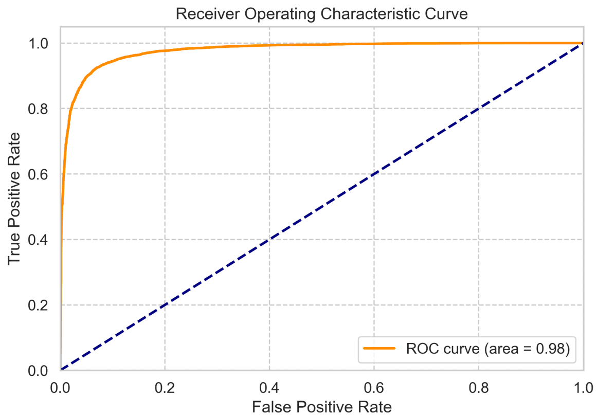
Figure 24: ROC Curve with AUC
