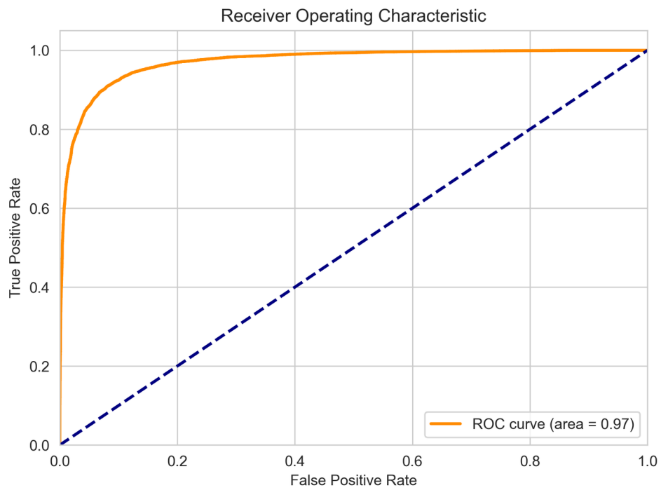
Figure 17: LinearSVC ROC Curve with AUC
