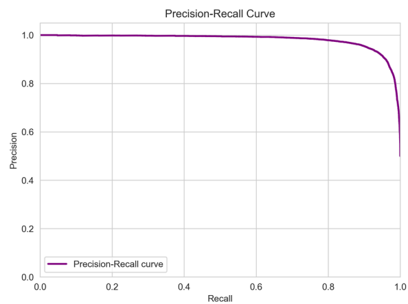
Figure 21: DistilBERT Precision-Recall curve
