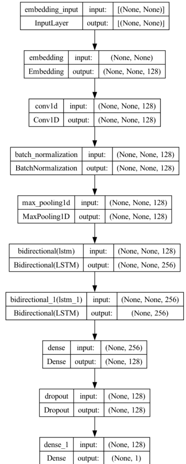
(c) Neural Network Architecture
