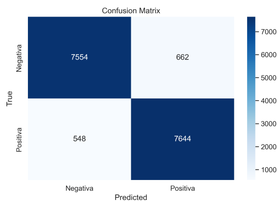
Figure 19: DistilBERT Confusion Matrix
