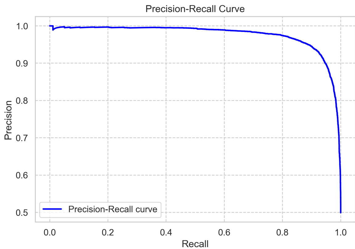
Figure 25: Precision-Recall Curve
