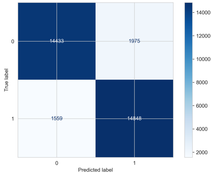
Figure 12: Confusion Matrix
