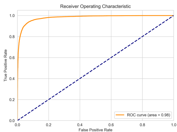
Figure 20: DistilBERT ROC Curve with AUC
