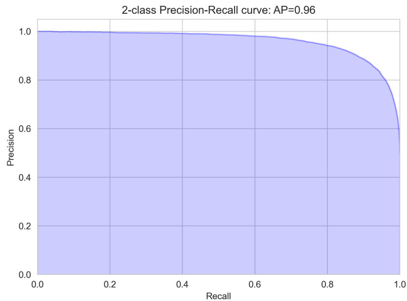
Figure 14: Precision-Recall curve
