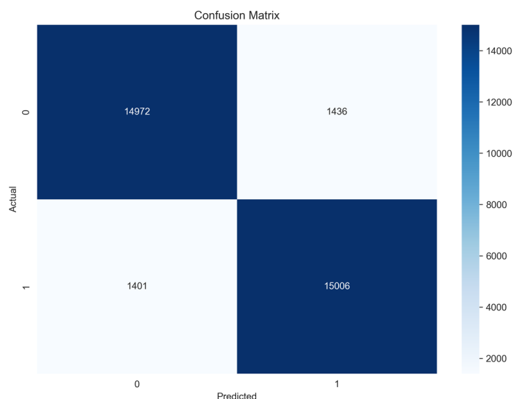
Figure 16: LinearSVC Confusion Matrix
