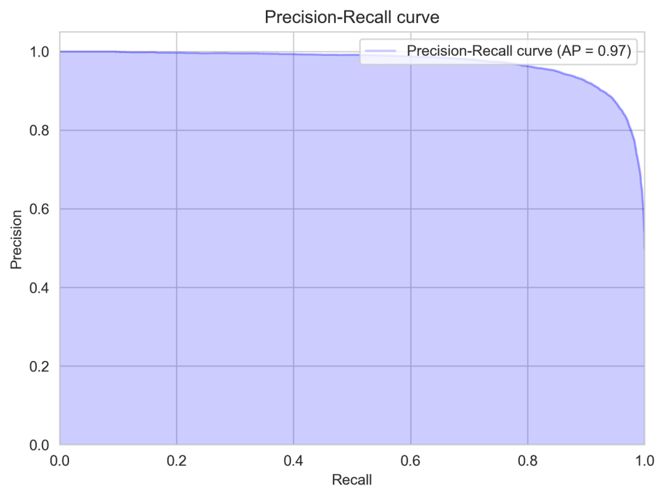
Figure 18: LinearSVC Precision-Recall curve
