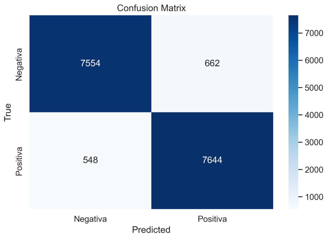
Figure 23: Confusion matrix
